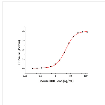
Immobilized Recombinant Rat VEGF164 at 1 \mu g/mL (100 \mu L/well) can bind Mouse KDR with a linear range of 0.03-4.7 ng/mL.
