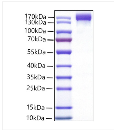
Recombinant Mouse VEGFR-2/KDR/CD309 Protein was determined by SDS-PAGE with Coomassie Blue, showing a band at 150-180kDa.
