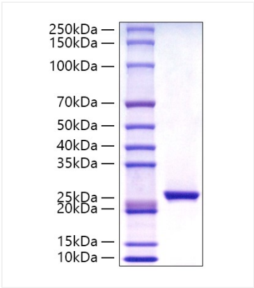
Recombinant Human C-Reactive Protein/CRP Protein was determined by SDS-PAGE with Coomassie Blue, showing a band at 25-30 kDa.
